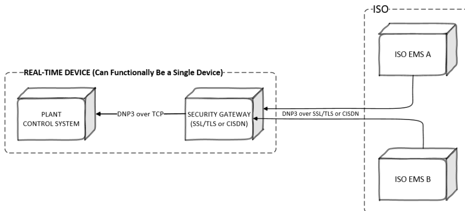
Exhibit 5-7: Plant Control System Hardware Option
