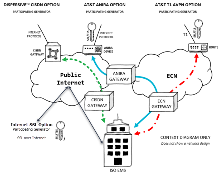
Exhibit 4-1: Context Diagram for Communications Options for Direct Telemetry
