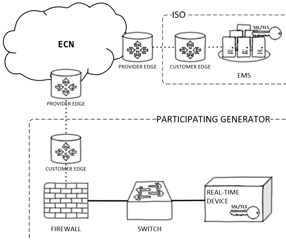
Exhibit 5-3: Transport Option – ECN with T1 Leased Circuit
