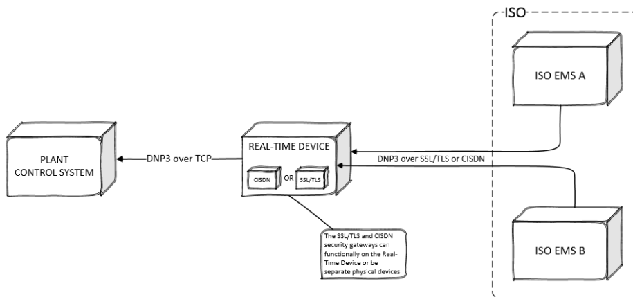
Exhibit 5-9: Real-Time Device Hardware Option
